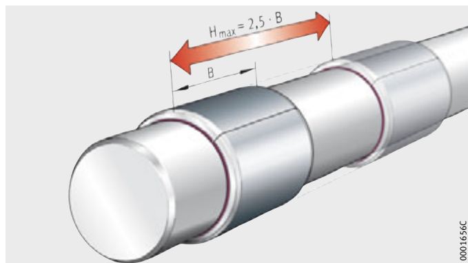
Figure 8 Correction factor for linear motion
