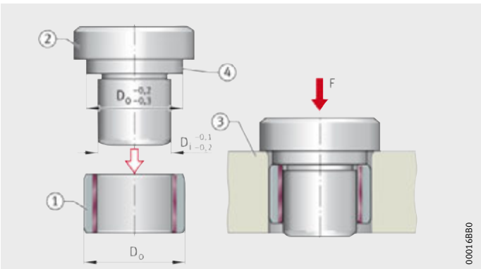
Figure 2 Pressing bushes into a counterbore
