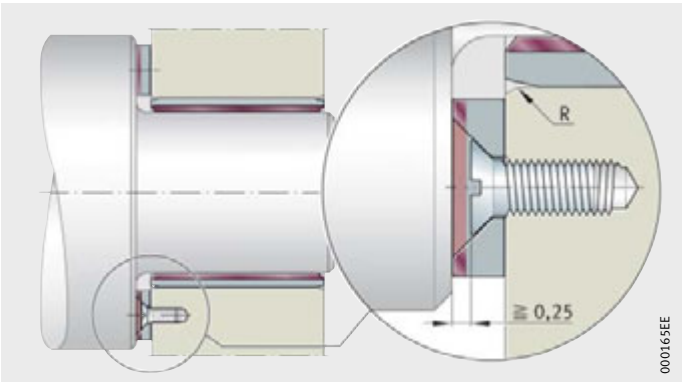
Figure 4 Prevention of rotation by countersunk head screw
