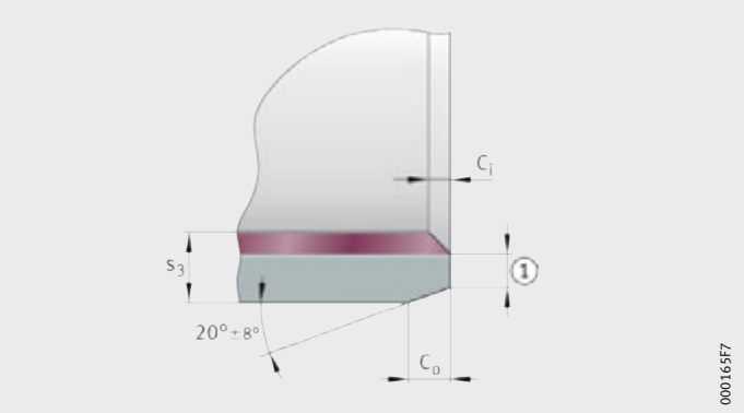
Figure 2 Outer chamfer and inner edge break
