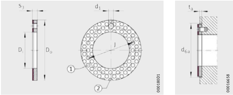
EGW ① Lubrication pockets, ② cutout 1)
